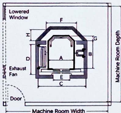
HOISTWAY MACHINE ROOM PLAN (ALTERNATE)
