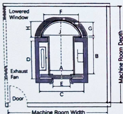
HOISTWAY MACHINE ROOM PLAN FOR CAPSULE ELEVATOR
